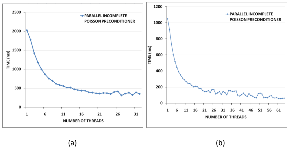
Figure 2: Parallelization results on multi-core hardware. (a) 8-core machine. (b) 32-core machine.
