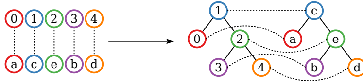
Figure 3.9: Relabelling
