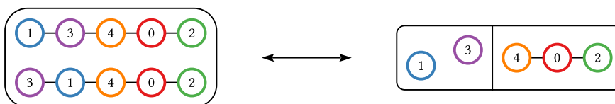
Figure 4.39: Isomorphism between L_{\geq 2}/\mathbb{Z}_2 and E_2 \cdot L
