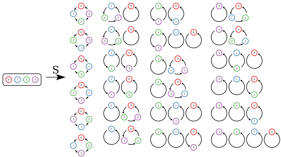
Figure 3.7: The species S of permutations
