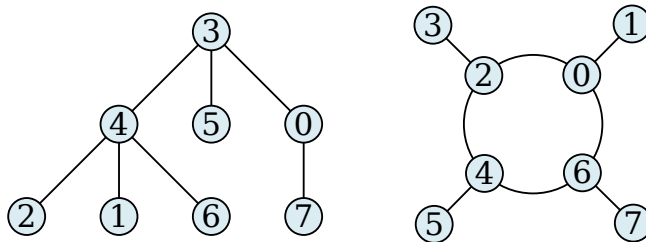
Figure 3.1: Representative labelled shapes
