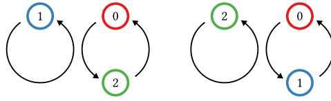
Figure 3.12: Two permutations with the same form
