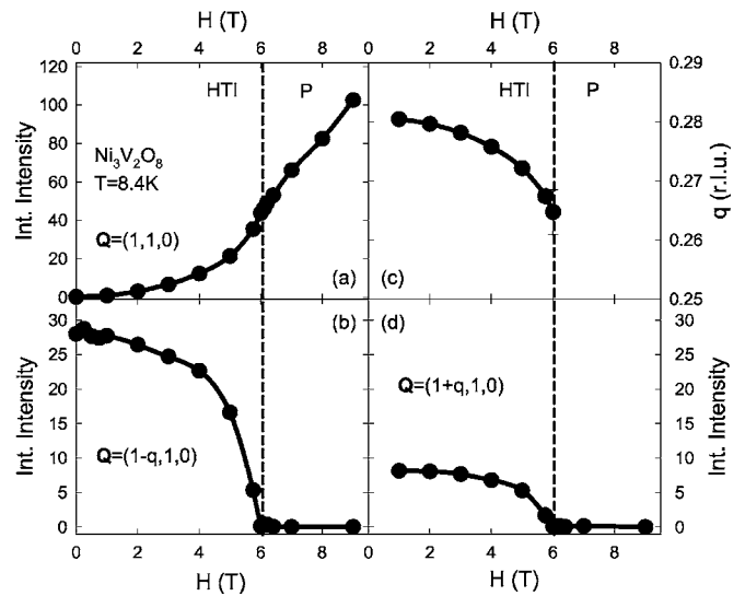
FIG. 14. Field dependence of magnetic Bragg peaks at T=8.4\text{ K} . Integrated intensities were obtained as for Fig. 12. Field dependence of the integrated intensity of (a) the AF (1, 1, 0) reflection, (b) the incommensurate (1-q, 1, 0) reflection, and (d) the incommensurate (1+q, 1, 0) reflection. (c) shows the field dependence of the incommensurate wave vector q .
