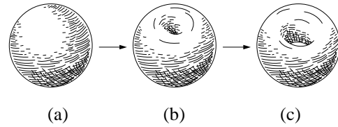
Figure 11: Hole evolution example
