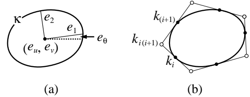
Figure 29: Ellipse-shaped blending regions
