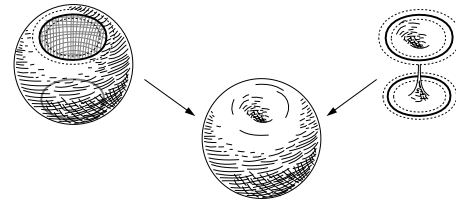
Figure 12: Pinched sphere construction
