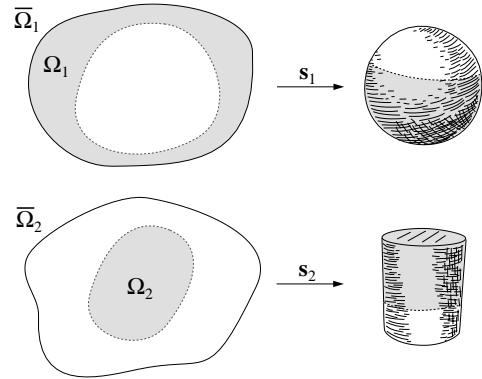
Figure 2: Underlying shapes s_1: \overline{\Omega}_1 \mapsto \mathbb{R}^3 ; s_2: \overline{\Omega}_2 \mapsto \mathbb{R}^3
