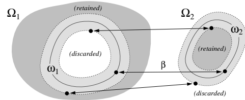
Figure 6: Annulus-shaped regions with correspondence \beta
