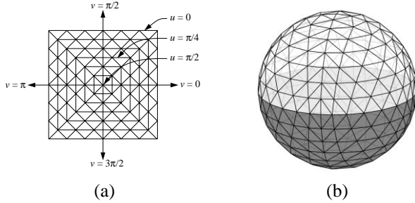
Figure 30: Split superellipsoid and half of its domain
