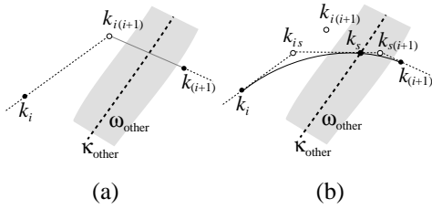
Figure 28: Region crossing example
