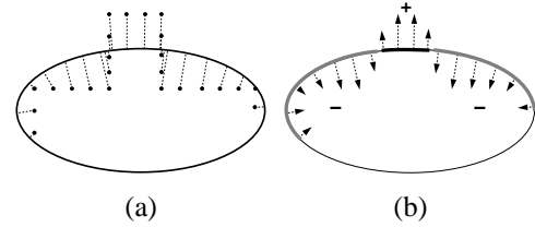
Figure 15: Model forces during equilibration
