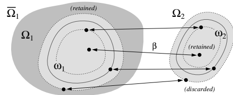
Figure 7: Disk-shaped regions with correspondence \beta
