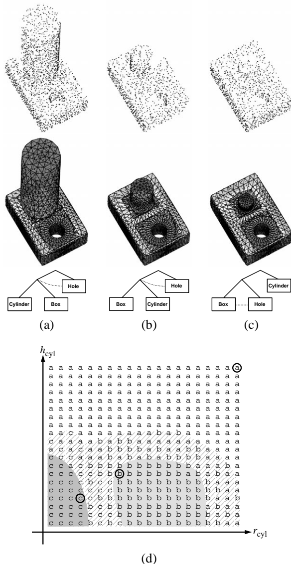
Figure 24: Various cylinder sizes in box/cylinder/hole object
