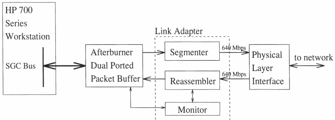
Figure 2: ATM Link Adapter
