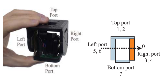
Fig. 2. One CKbot module with a schematic representation. The arrow indicates the rotational axis, the numbers are the port identification numbers assigned to each port
