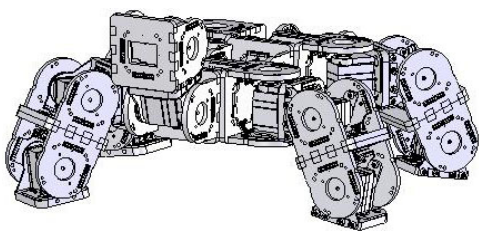
Fig. 1. Surveyor Dog 17 modules in a 4-legged configuration
