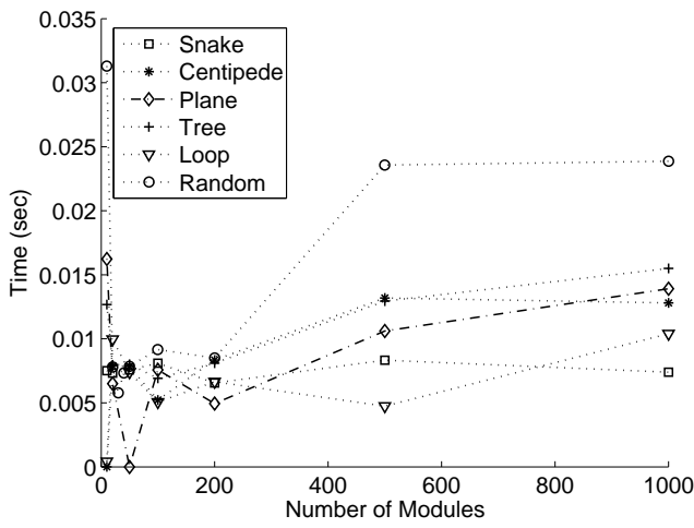
Fig. 19. Standard deviation of search times for 3DLL vs. number of modules in robot configuration.
