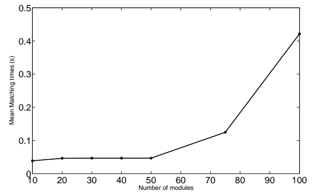
Fig. 7. Mean search times for nauty based algorithm vs. number of modules in robot configuration.
