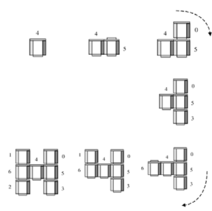
Fig. 17. Building a linked list based representation for a modular robot.
