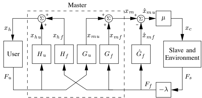
Fig. 3. Induced master motion can be canceled using the model \hat{G}_f .
