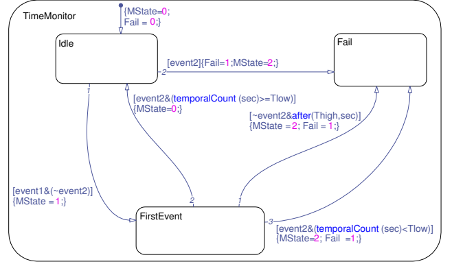
Figure 14. Design of a monitor used to check timing dependencies between events.
