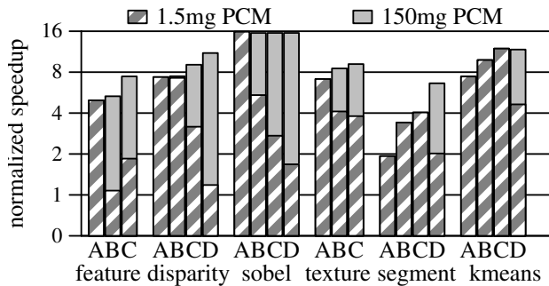
Figure 9. Speedup on 16 cores with varying input sizes
