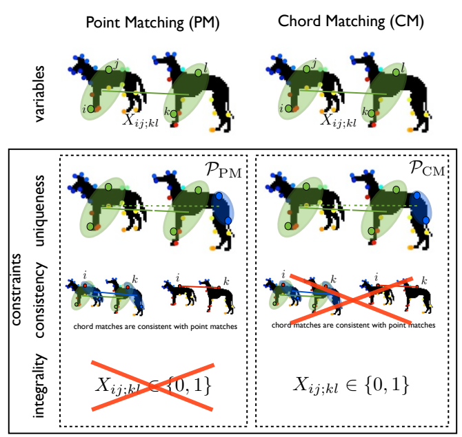
Fig. 10 Relaxation of GMC. Left: Point Matching (PM) is obtained by relaxing the integrality constraint. Right: Chord Matching (CM) is obtained by relaxing the consistency constraints.
