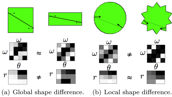
Fig. 4 For each pair of shapes (upper row), we show two chord diagrams: one computed over the normal features only (middle row) and one over the chord length and orientation (lower row).
