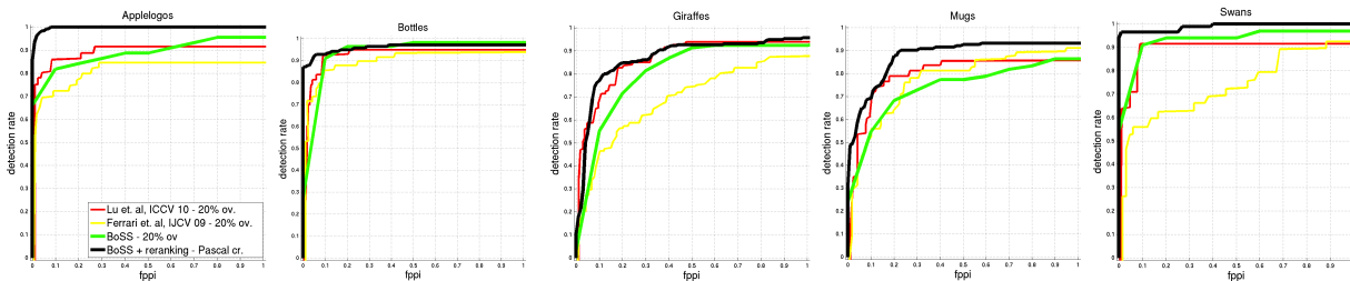
(a) detection rate vs false positives per image (fppi)
