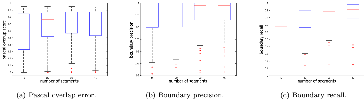
Fig. 22 We present three different measures for the quality of the segmentation. For each measure, we use all images from the ETHZ Shape Dataset and pre-segmentations with 10, 20, 30, and 45 segments. We display for each measure and pre-segmentation, the median in red, the 25% and 75% quantile as blue boxes, and the range of the values as black lines.
