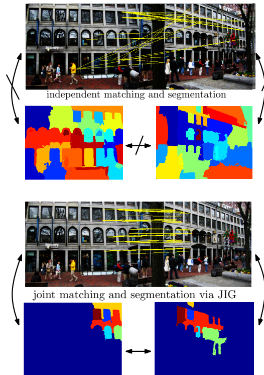
Figure 1. Independently computed correspondences and segments (upper diagram) for a pair of images can be made consistent with each other via the joint image graph and thus improved (lower diagram).
