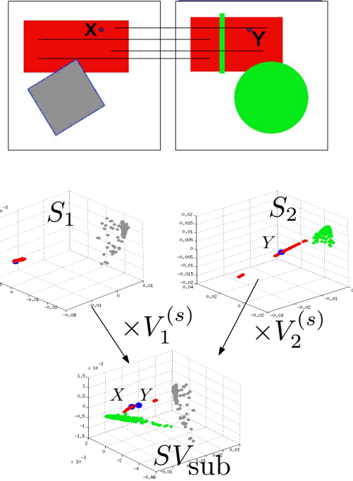
Figure 4. Subspace view of the segmentation synchronization. Below each of the images in the first row, the embedding of the pixels of the image in the segmentation space spanned by the top 3 eigenvectors is displayed. The pixels coming from different objects in the image are encoded with the same color. In the third row, both embeddings transformed by the optimal V_{\text{sub}} (eq. (6)) are presented, given the matches selected as shown in the first row. Both embeddings were synchronized such that all pixels from both rectangles form a well grouped cluster (the red points). In this way the matches were correctly extended over the whole object, even in presence of an occlusion (green vertical line in right image).
