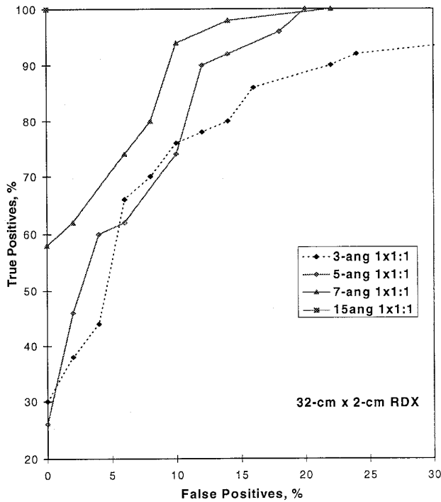
Fig. 6. ROC curves showing the effect of varying the number of projection angles used in the tomographic reconstruction. The reconstruction used a pixel resolution of 1-cm by 1-cm and a projection resolution of 1 cm. Note the single 15-angle point is located in the upper left-hand corner.
