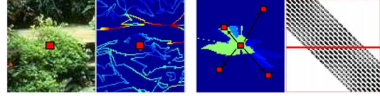
Figure 1: Column 1 and 2: image and image edges. Column 3 and 4: segmentation graph encoding intervening contour grouping cue. Two pixels have high affinity if the straight line connecting them does not cross an image edge. Column 3 displays one row W_C(i, :) of the graph connection matrix reshaped as an image, for the central pixel i . The row corresponds to the red line on column 4.
