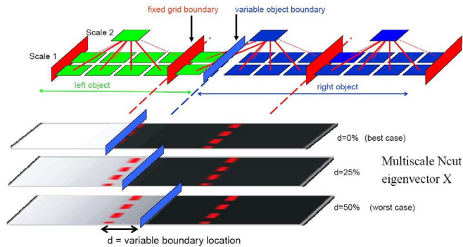
Figure 10: Non-adaptive grid can produce precise object boundaries and recover from errors in grid quantization. Top: a two level graph, with coarse nodes spaced on a regular grid (boundaries in red). An object boundary (in blue) specifies two regions (green vs. blue) with low mutual affinity. Its location d (as % of grid size) w.r.t. the grid varies from d = 0\% (best case, grid and object boundaries agree) to d = 50\% (worst case, object boundary cuts the grid in half). The central coarse node is linked either to left or right coarse nodes depending on d . Bottom: multiscale Ncut eigenvector for d = 0\% , 25\% , 50\% . In all cases, multiscale segmentation recovers from errors in coarse level grid. Notice that the gap in Ncut eigenvector across the object boundary remains high even in worst case.
