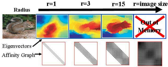
Figure 2: The Ncut segmentation eigenvector of the left image for increasingly large graph connection radius G_r . With larger G_r , the squirrel with faint contours pops out more clearly, but the graph affinity matrix becomes denser. The bottom row shows zoomed out versions of the affinity matrices.
