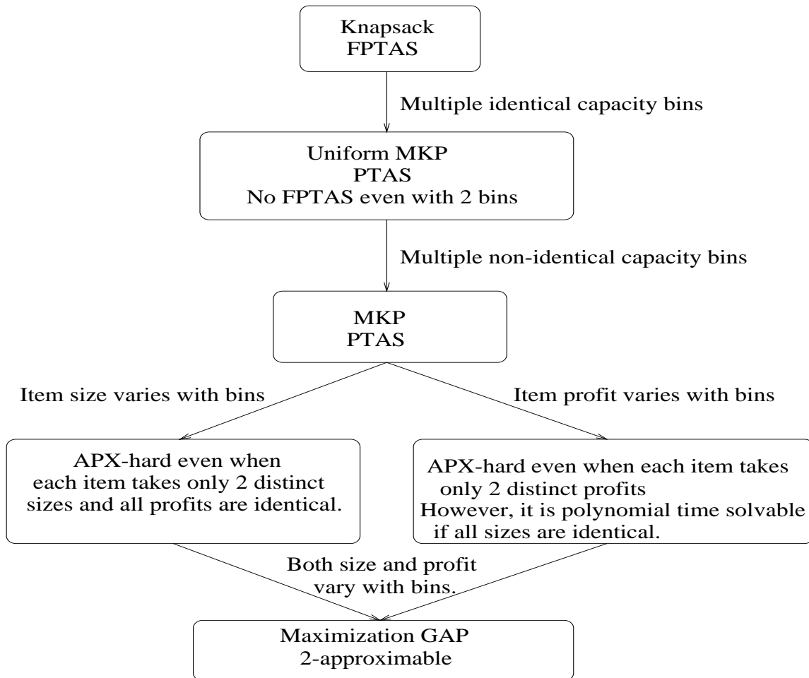
Figure 1: Complexity of Various Restrictions of GAP
