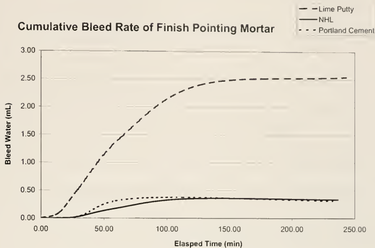
Graph 5.5. Cumulative Bleeding Rates of Finish Pointing Mortar
