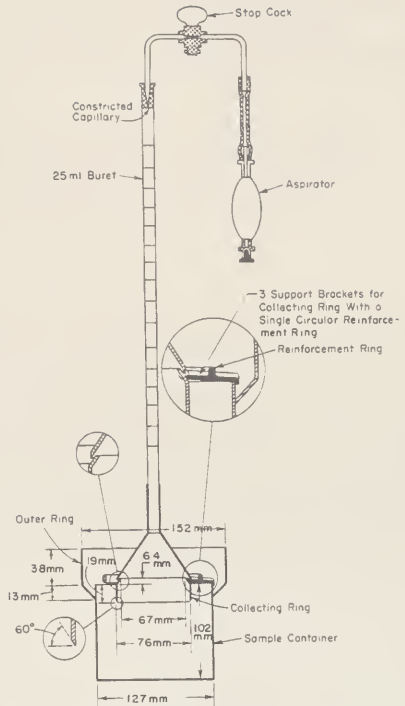
Figure 2.3. Diagram of the Liquid Displacement Bleeding Apparatus required for ASTM C 243-95.
