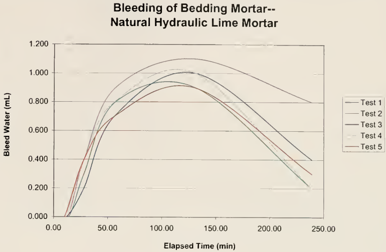
Graph 3.6. Bleeding Rate—1 Natural Hydraulic Lime: 0.5 Brick Dust: 2.5 Sand
