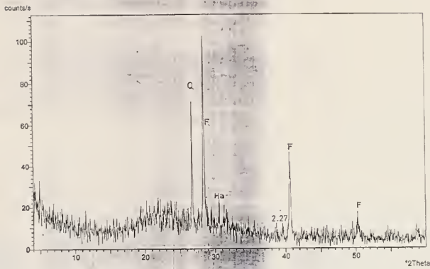
Figure 3: The X-ray diffraction patterns of the wood ash. Provenance: Qven from farmers at Abu Nomros AKCS-E (lab code 359/02)
