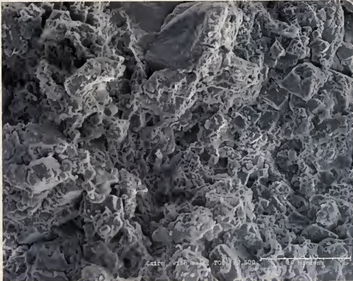
Figure 6.12. Egyptian Limestone Sample Impregnated with Sodium Chloride, Brushed with Triton, Poulitced with Orvus. 2,500x magnification
