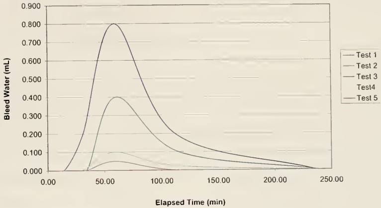
Graph 4.8. Cumulative Bleeding Rate—1 Portland Cement: 3 Dry Mixture
