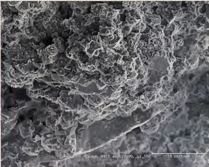
Figure 6.8. Egyptian Limestone Sample Impregnated with Sodium Chloride, Brushed with Orvus, Poulticed with Orvus. 2,500x magnification
