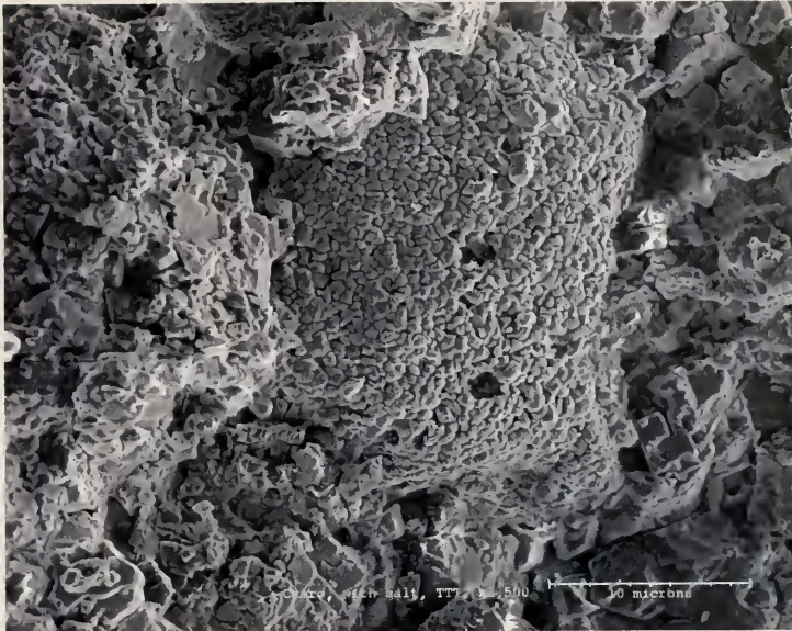
Figure 6.11. Egyptian Limestone Sample Impregnated with Sodium Chloride, Brushed with Triton, Poulitced with Triton. 2,500x magnification
