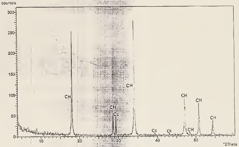
Figure 1: The X-ray diffraction patterns of the lime putty, 3-4 months in water AKCS-E (lab code 351/02)
