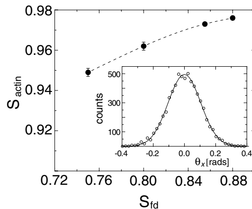
FIG. 2. The order parameter of actin filaments ( S_{actin} ) vs the order parameter of the background fd nematic ( S_{fd} ). Dashed line is a guide to the eye. The contour length of actin filaments is 15 \mu m or higher. The values of S_{fd} at different fd concentrations have been measured in Ref. [14]. Inset: The orientational distribution function (ODF) of actin filaments. The ODF is well approximated by a Gaussian distribution for a wide range of concentrations.
