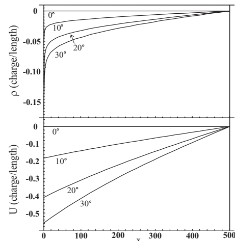
FIG. 4. Equilibrium solutions for a piezoelectric tube in the electrostatically dominated limit using the soft kernel. The upper panel shows the induced bound charge density for tubes of various chiralities, while the lower panel shows the corresponding electrostatic potential along the tube. The graphs were generated using \beta=1 , \lambda_1=1000 , \lambda_2=10000/\pi , \lambda_3=2\lambda_2 , and e_2=\sqrt{5000}/\pi (charge/length).
