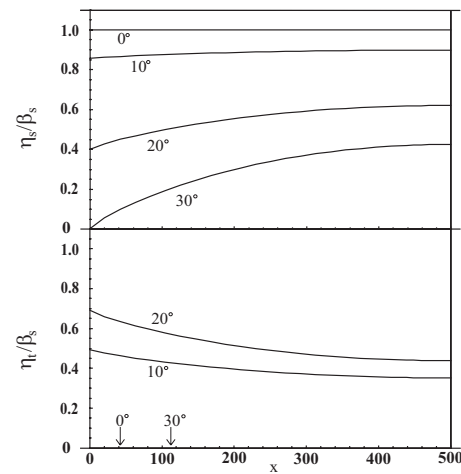
FIG. 3. Equilibrium solutions for a piezoelectric tube in the electrostatically dominated limit using the soft kernel. The upper panel shows the induced uniaxial strain for tubes of various chiralities, while the lower panel shows the corresponding induced torsional strains. The graphs were generated using \beta=1 , \lambda_1=1000 , \lambda_2=10000/\pi , \lambda_3=2\lambda_2 , and e_2=\sqrt{5000}/\pi (charge/length).
