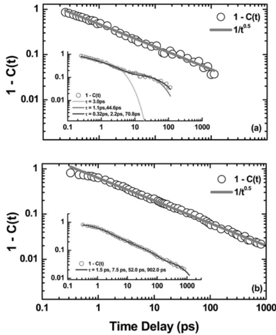
FIG. 3. (a) 1-C(t) (open circles) versus t on a log-log scale for an (8,6) tube. 1-C(t) is linear over three decades in time and shows 1/\sqrt{t} dependence. y=1/\sqrt{t} (line) is shown for comparison. (inset) 1-C(t) compared to mono-, bi-, and tri-exponential fits. (b) Similar linear behavior is observed for a (7,6). (inset) A good fit now requires at least four exponentials.
