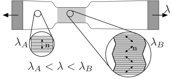
FIG. 7. An illustration of a possible microstructure that would result from the applied in-plane deformation. Depending on the cost of the interface, the disproportionation illustrated here may happen in several regions in the sample. The region where the microstructure forms may be opaque as illustrated.
