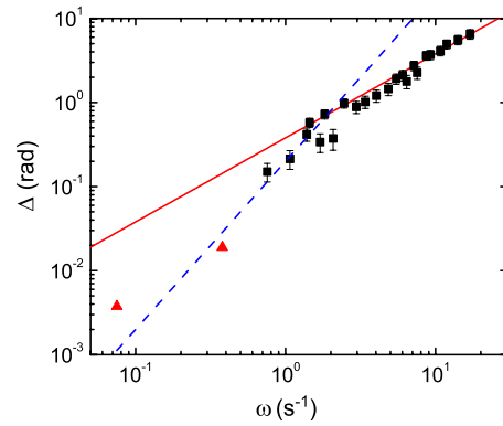
FIG. 10. (Color online) Total phase difference \Delta plotted as a function of the driving frequency \omega for the bubble raft experiments (black squares). The two triangles represent an upper limit for the measured phase-shift given the resolution of our experiment at the corresponding frequencies. The solid and dashed lines have slopes 1 and 2, respectively. The intersection of these two lines provides a rough estimate for the crossover frequency, \omega_p \approx 1.9 \pm 0.9 \text{ s}^{-1} .
