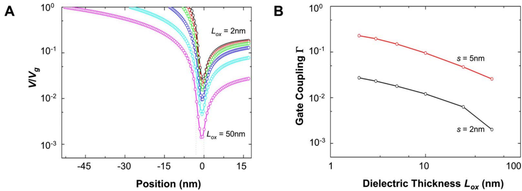
FIG. 7. (Color online) Electrodes with nonuniform cross section—role of the dielectric thickness. (a) Normalized potential for the three-dimensional device shown in Fig. 4(a) with t=3\text{ nm} , s=2\text{ nm} , \theta=120^\circ , \kappa=4 , values of L_{ox} from top to bottom are 2, 3, 5, 10, 25, and 50 nm; (b) Gate coupling as a function of dielectric thickness for the three-dimensional device shown in Fig. 4(a) with t=3\text{ nm} , \theta=120^\circ , \kappa=4 .
