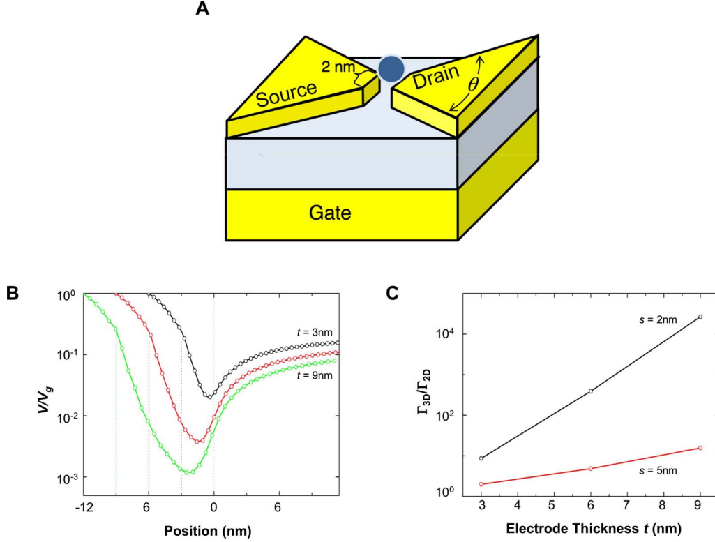
FIG. 4. (Color online) Electrodes with nonuniform cross section—role of the electrode thickness. (a) Schematic of a typical three-terminal molecular-scale electronic device fabricated using feedback controlled electromigration; (b) normalized potential for the three-dimensional device shown in A with L_{ox}=3 nm, s=2 nm, \kappa=4 , \theta=120^\circ , values of t from top to bottom are 3, 6, and 9 nm; (c) ratio between gate coupling factor \Gamma for 3D electrodes with \theta=120^\circ and for 2D electrodes, both with L_{ox}=3 nm, \kappa=4 .
