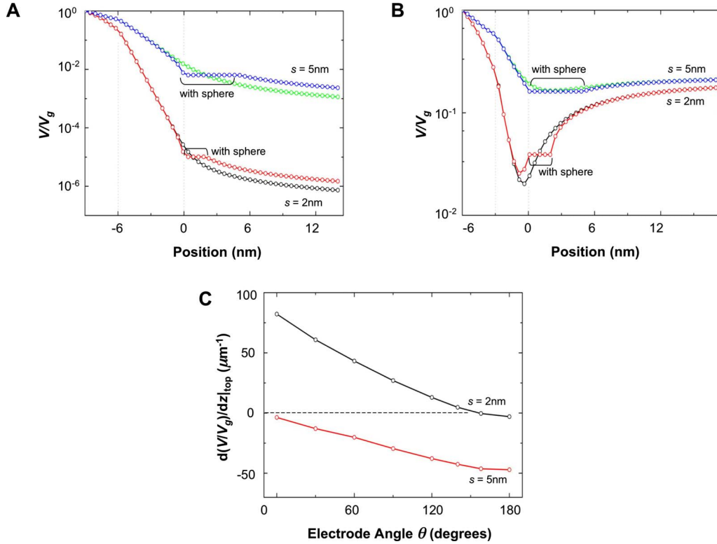
FIG. 8. (Color online) Electrodes with uniform and nonuniform cross section—effect of molecular polarizability. (a) Normalized potential for the two-dimensional device shown in Fig. 1(a) with L_{ox}=3\text{ nm} , t=6\text{ nm} , \kappa=4 , for bare electrodes and electrodes with a polarizable sphere of diameter s and \kappa=10^6 positioned at the top of the nanogap; (b) Normalized potential for the three-dimensional device shown in Fig. 4(a) with L_{ox}=3\text{ nm} , t=3\text{ nm} , \kappa=4 , for bare electrodes and electrodes with a polarizable sphere of diameter s and \kappa=10^6 positioned at the top of the nanogap; (c) derivative of the normalized potential with respect to vertical position for the three-dimensional device shown in Fig. 4(a) with L_{ox}=3\text{ nm} , t=3\text{ nm} , \kappa=4 .
