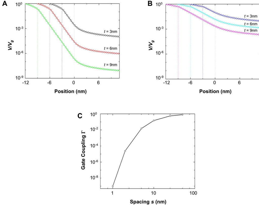
FIG. 3. (Color online) Electrodes with uniform cross-section—roles of the electrode thickness and spacing. (a) Normalized potential for the two-dimensional device shown in Fig. 1(a) with L_{ox}=3 nm, s=2 nm, \kappa=4 ; (b) Normalized potential for the two-dimensional device shown in Fig. 1(a) with L_{ox}=3 nm, s=5 nm, \kappa=4 ; (c) gate coupling as a function of nanogap size for the two-dimensional device shown in Fig. 1(a) with L_{ox}=3 nm, t=6 nm, \kappa=4 .
