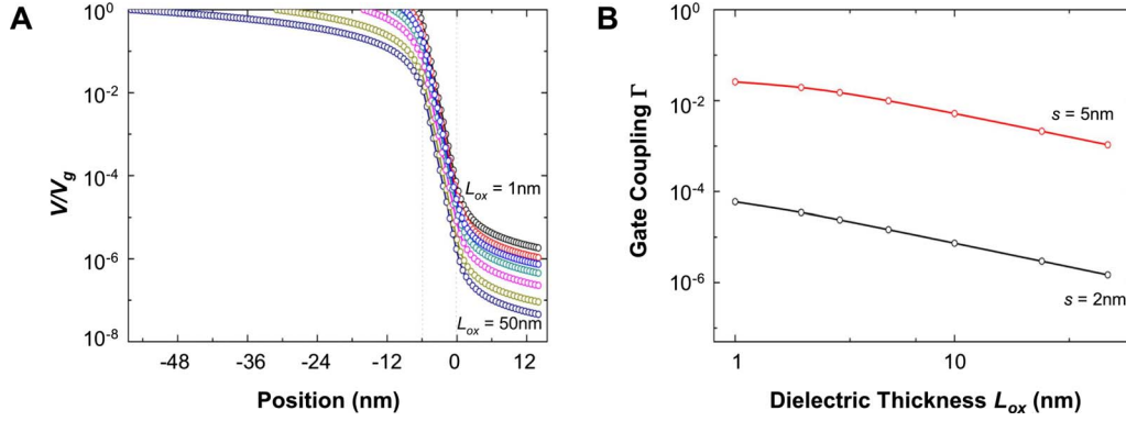
FIG. 2. (Color online) Electrodes with uniform cross-section—role of the dielectric thickness. (a) Normalized potential for the two-dimensional device shown in Fig. 1(a) with t=6 nm, s=2 nm, \kappa=4 , values of L_{ox} from top to bottom are 1, 2, 3, 5, 10, 25, and 50 nm; (b) Gate coupling as a function of dielectric thickness for the two-dimensional device shown in Fig. 1(a) with t=6 nm, \kappa=4 .
