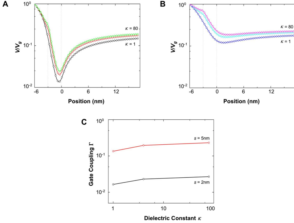
FIG. 6. (Color online) Electrodes with nonuniform cross section—role of the dielectric constant. (a) Normalized potential for the three-dimensional device shown in Fig. 4(a) with L_{ox}=3\text{ nm} , t=3\text{ nm} , s=2\text{ nm} , \theta=120^\circ , values of \kappa from bottom to top are 1, 4, and 80; (b) Normalized potential for the three-dimensional device shown in Fig. 4(a) with L_{ox}=3\text{ nm} , t=3\text{ nm} , s=5\text{ nm} , \theta=120^\circ , values of \kappa from bottom to top are 1, 4, and 80; (c) Gate coupling for the three-dimensional device shown in Fig. 4(a) with L_{ox}=3\text{ nm} , t=3\text{ nm} , \theta=120^\circ .
