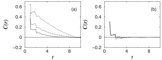
FIG. 6. Spatial correlation function C(r) of particle vibrations at three values of \Delta\phi = 10^{-6} (solid line), 10^{-2} (dashed), and 10^{-1} (dotted), for N=10\,000 monodisperse spheres in 3D, averaged over (a) the ten lowest-lying frequency modes, and (b) ten modes at intermediate frequencies \omega \sim 0.5 .
