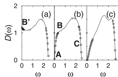
FIG. 1. Density of states D(\omega) of 3D jammed packings of monodisperse spheres at three different compressions \Delta\phi=(a) 10^{-6} , (b) 10^{-2} , and (c) 10^{-1} . In (a) we identify regime B' , and in (b) we identify the regimes A , B , and C discussed in the text. The lines show data for the systems with N=1024 . The symbols show the low- and high-frequency portions of D(\omega) for N=10\,000 . There is no discernible size dependence.
