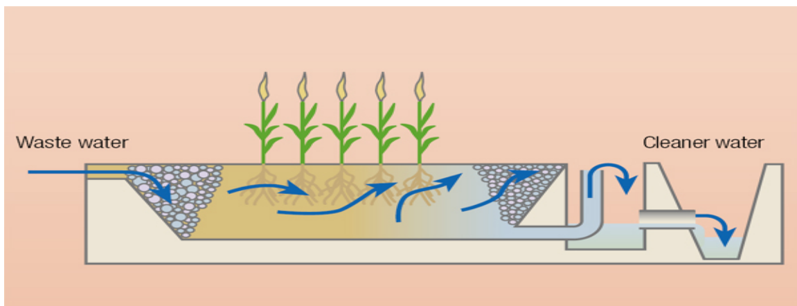
Fig. 5 – Example of a constructed wetland for AMD Source: United Nations Environment Program http://www.unep.org/geo/yearbook/yb2003/images/fresh_img_g_40.jpg
