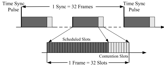
Figure 3: RT-Link time slot allocation with out-of-band synchronization pulses
