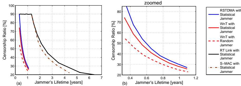
Figure 14: (a) Dependency between jammer's lifetime and Censorship Ratio and (b) zoomed
