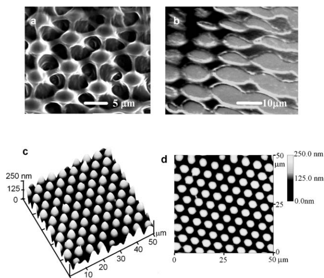
Fig. 2 Hydrogel microlens arrays formed from poly(2-hydroxyethyl methacrylate- co -methyl methacrylate) by interference lithography. (a,b) SEM images of (a) non-deformed and (b) highly deformed microlens arrays. (c,d) Atomic force micrographs (AFM) of the topography of hydrogel lens arrays shown in (a) side (c) and top (d) views.
