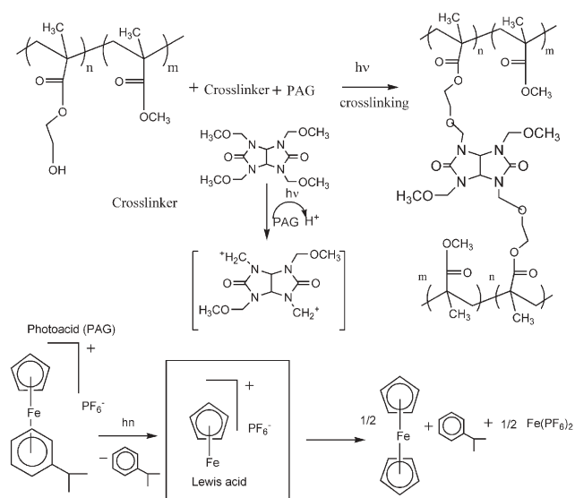
Scheme 1 Schematic illustration of photoacid generation and crosslinking reaction in poly(2-hydroxyethyl methacrylate- co -methyl methacrylate).
