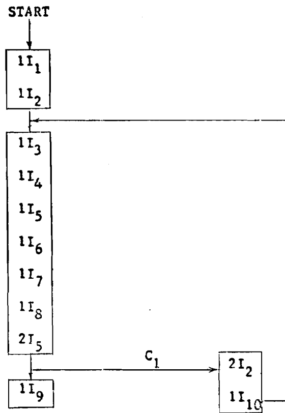
Figure 8. Moore-type representation of factorial program
