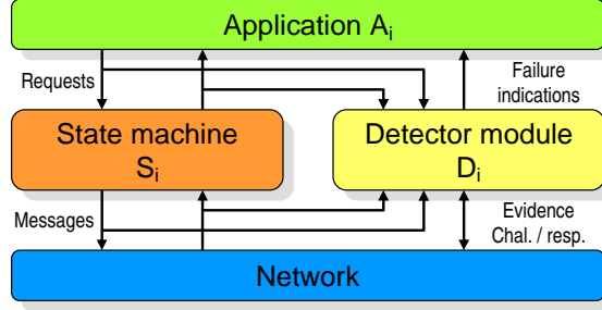
Figure 7: Architectural Model of Node i
