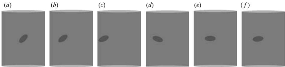
FIGURE 23. Transient motion of a spheroid settling in a tube at a Reynolds number around 1.0. Initial orientation of the spheroid is \beta = -45^\circ . The aspect ratio of the spheroid is a/b = 2.0 and the tube diameter D = 8a . The density ratio \rho_p/\rho_f = 1.5 .
