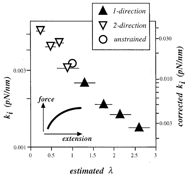
FIGURE 10 Effective spring constant versus estimated network extension ratio ( \lambda ). Network stretches in the 1- or 2-directions were estimated (together with \pm SD) from results of the type illustrated in Fig. 7 and were applied to each datapoint of measured fluctuations (Fig. 8). Directional spring constants were determined from the equipartition theorem per Eq. 5b either with or without noted corrections of the r.m.s. displacements (see Appendix 1). The gray region corresponds to the elasticity error introduced by the \pm 6 nm SD in the measured bead motions on the unstrained portion of the cell; the vertical error bars of Fig. 8 are otherwise omitted. The inset sketch of force versus extension schematically indicates the continuous strain softening that is clearly implicated by the reduced spring constant ( k_{SP} \sim df/d\lambda ).
