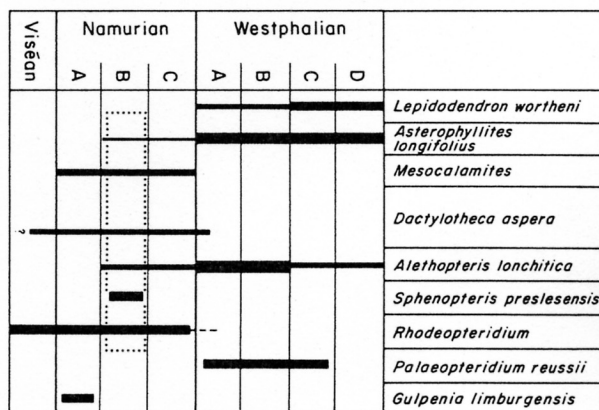
Text fig. 13 - Stratigraphic ranges in the European Carboniferous of genera and species occurring in the Spencer Farm Flora. (Data from Gothan and Remy (1957), Fossilium Catalogus, and other sources.) Dotted outline shows time of common occurrence of the majority of forms.
