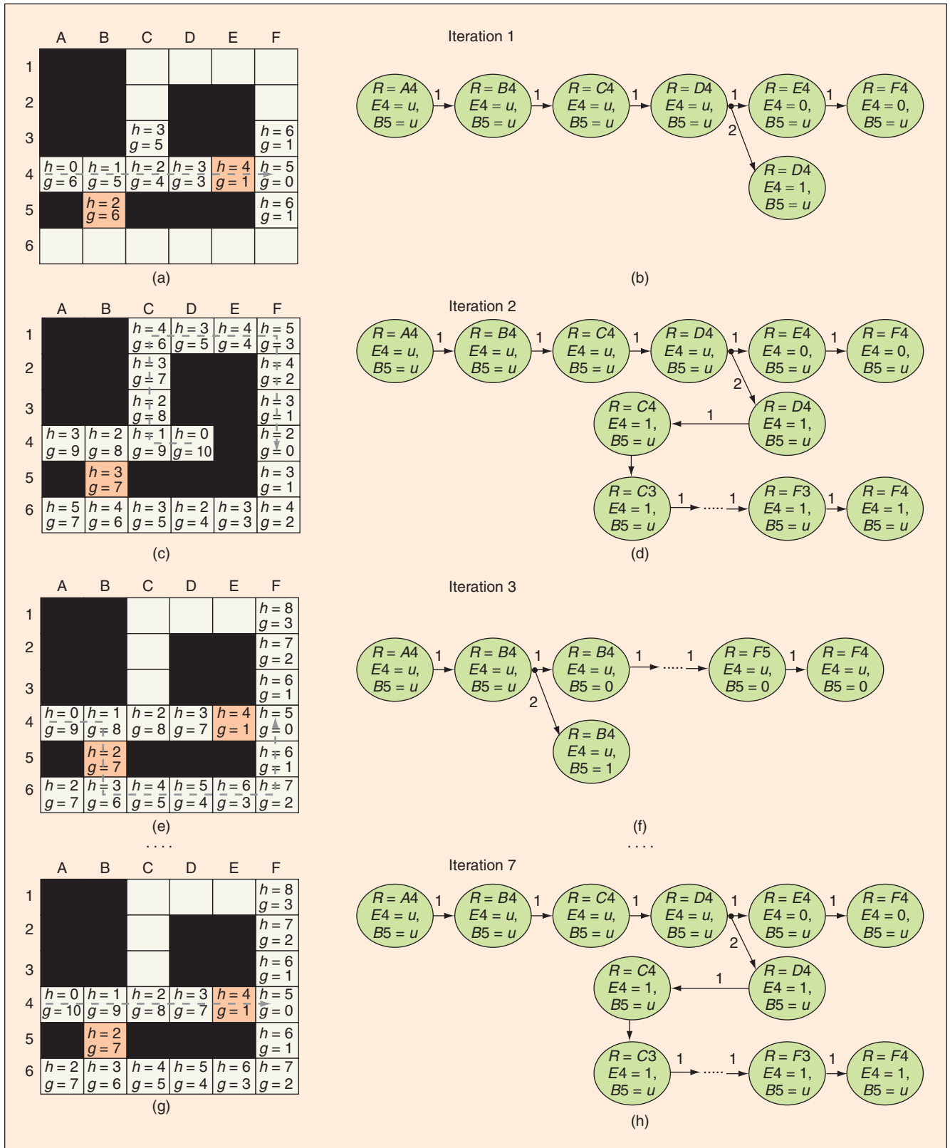
Figure 4. Example of how PPCP operates. (a) Search for a path from [R = A4; E4 = u, B5 = u] . (b) PPCP policy after update. (c) Search for a path from [R = D4; E4 = 1, B5 = u] . (d) PPCP policy after update. (e) Search for a path from [R = A4; E4 = u, B5 = u] . (f) PPCP policy after update. (g) Search for a path from [R = A4; E4 = u, B5 = u] . (h) Final PPCP policy.
