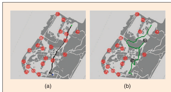
Figure 2. Solving the path clearance problem with freespace assumption. (a) Planned path. (b) Actual path of the agent.
