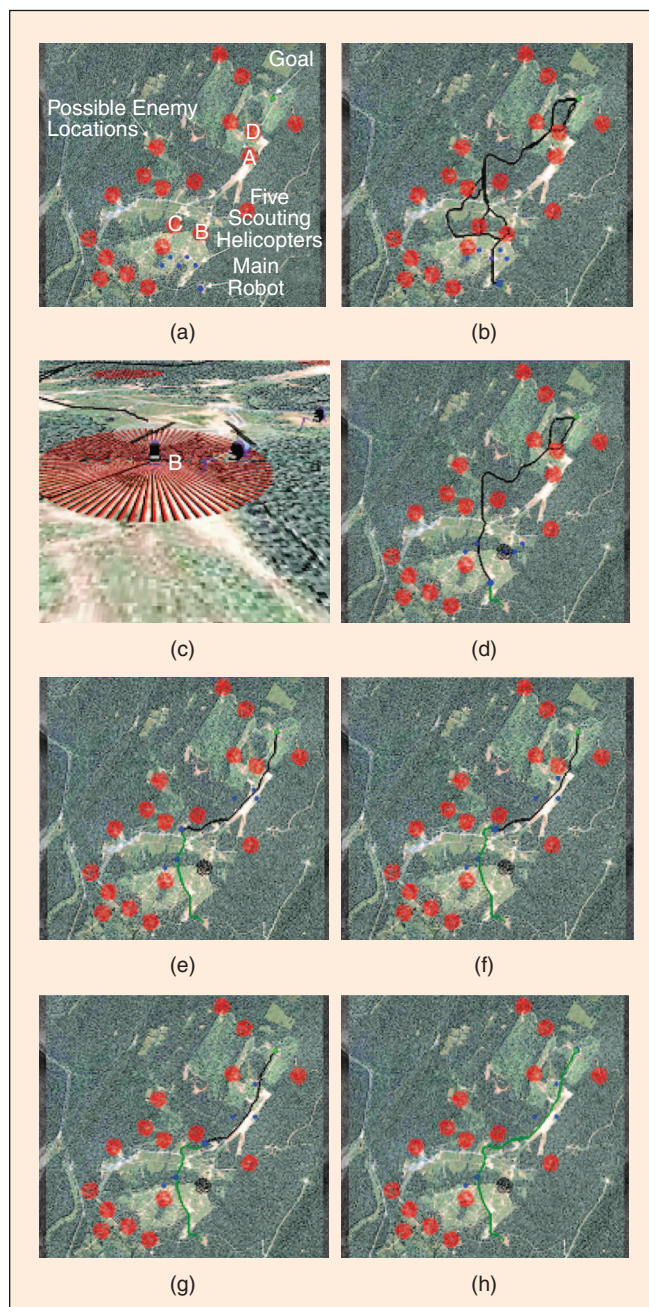
Figure 8. Path clearance with PPCP planning and information value-driven use of five scouts. (a) Initial configuration. (b) Plan after convergence (30 s). (c) Scouting helicopters on mission. (d) Locations B and C sensed (adversary detected in B). (e) Location A sensed. (f) Scout moves toward D. (g) Location D sensed. (h) Agent reaches its goal.
