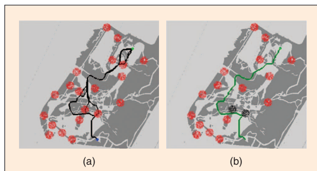
Figure 3. Solving the path clearance problem with PPCP. (a) Generated plan. (b) Actual path of the agent.
