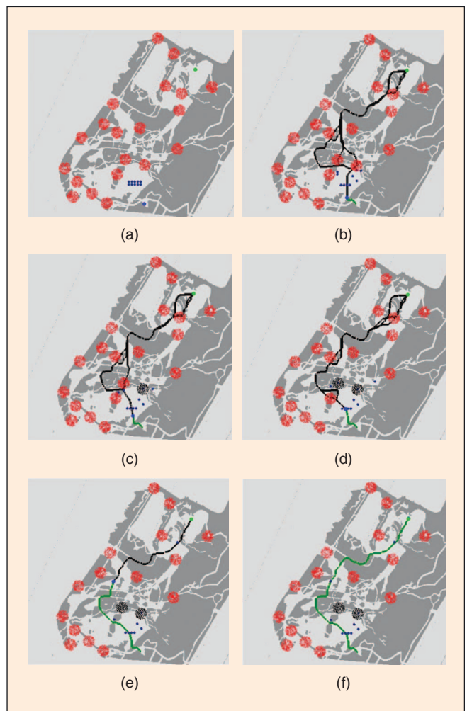
Figure 7. Path clearance with PPCP planning and likelihood-driven use of ten scouts. (a) Initial configuration. (b) Plan after convergence (30 s). (c) Location B sensed (adversary detected). (d) Location C sensed (adversary detected). (e) Location D sensed (no adversary present). (f) Agent reaches its goal.
