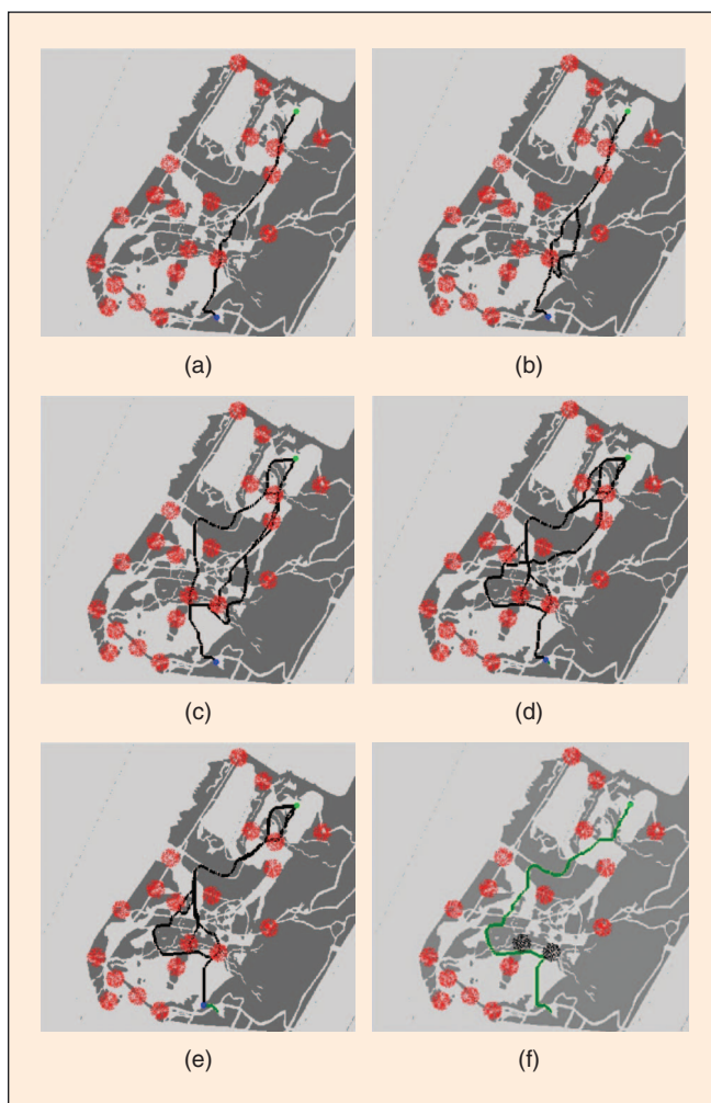
Figure 5. Applying PPCP to path clearance. (a) The first policy. (b) The second policy. (c) After 5 s. (d) After 15 s. (e) After 30 s (PPCP converged). (f) Actual path of the agent.
