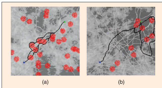
Figure 6. The example of environments used in testing and the plans generated by PPCP for each. (a) Typical Group I environment. (b) Typical Group II environment.
