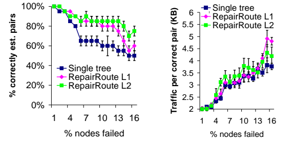
(a) Established join pairs (b) Total traffic Figure 9: Node failures
