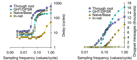
(a) Result delay (b) Result quality Figure 8: Increasing sampling rate
