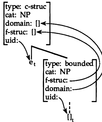
Figure 26: The complete simulation of (8). This is figure 24 with the domain feature added.
