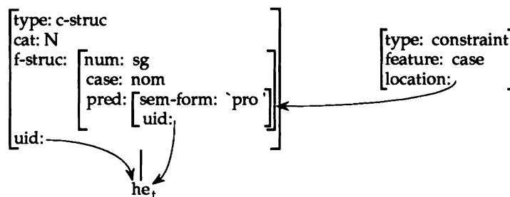
Figure 21: The simulation of (4), repeated below.
