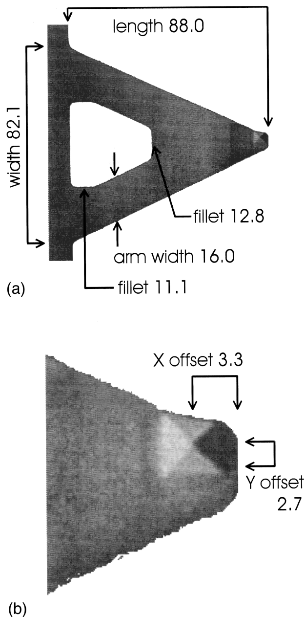
FIG. 2. (a) A scanning electron micrograph of a gold coated Park Scientific Instruments “F” cantilever. The indicated dimensions are in micrometers. (b) A higher magnification view of the end of the lever, showing the position of the tip (at the apex of the pyramid) relative to the lever. The tip is off-axis by an amount close to its nominal height of 3 \mu\text{m} , which is an additional source of coupling between normal and lateral forces.
