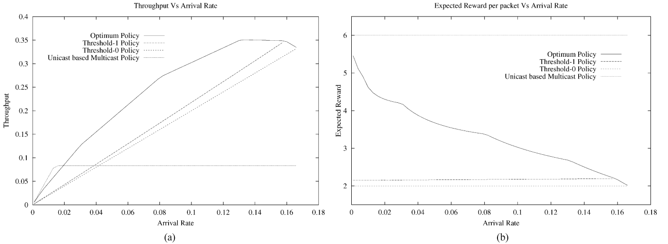
Fig. 8. The throughput and the expected reward per packet of various multiple-access multicast strategies as a function of the arrival rate. Here, optimum policy refers to the two-threshold policy \Delta^* that maximizes the throughput subject to stability. (a) Throughput versus \lambda . (b) Expected reward per packet versus \lambda .
