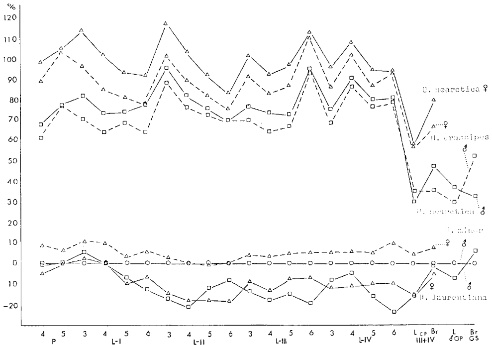
FIGURE 16. Ratio diagram comparing Unionicola laurentiana , n. sp. (below) and U. nearctica n. sp. (above) with U. minor and U. crassipes . ○ = U. minor ♂♂; △ = ♀♀; □ = ♂♂; broken lines = U. crassipes (above) and U. minor ♀♀ (below).
