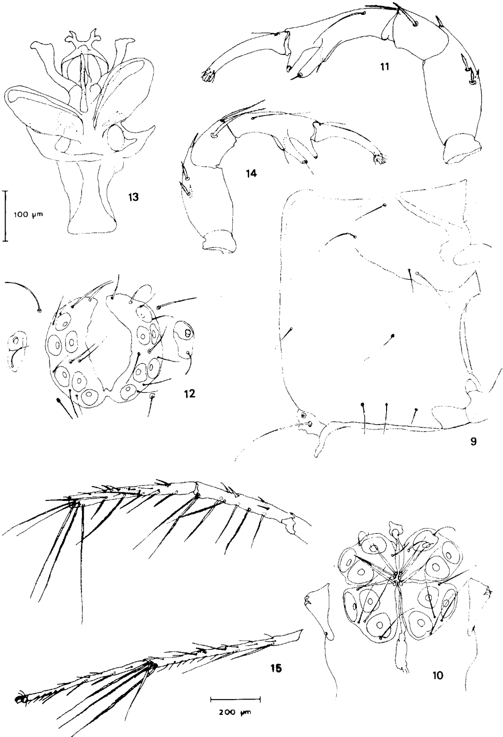
FIGURES 9-15. Unionicola nearctica , n. sp. (scale equals 100 μm) 9. ♀ coxae III+IV. 10. ♀ genital plates. 11. ♀ left palp, lateral view. 12. ♂ genital plates. 13. ♂ genital skeleton. 14. ♂ right palp, lateral view. 15. (scale equals 200 μm) leg IV, posterior view.
