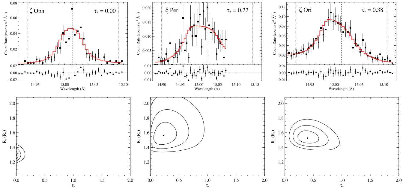
Figure 1. The Fe XVII line at 15.014 Å with best-fitting model (top row) for three of the sample stars [ \zeta Oph, \tau_* = 0.00^{+0.01}_{-0.00} (left), \xi Per, \tau_* = 0.22^{+0.14}_{-0.12} (middle) and \zeta Ori, \tau_* = 0.38^{+0.13}_{-0.11} (right)] showing various degrees of asymmetry. The vertical dashed lines on the profile plots represent the laboratory line rest wavelength and the wavelengths corresponding to the terminal velocity of the wind. Note that the x -axis in each figure in the top row encompasses the same velocity range in units of the wind terminal velocity, but different absolute velocity and wavelength ranges, due to the different terminal velocities of the three stars' winds. The star with the highest wind velocity, \xi Per, is subject to more blending on its red wing than are the other two stars. The contours in the lower panels give the 68, 95 and 99.7 per cent two-dimensional joint confidence limits on \tau_* and R_0 , while the best-fitting models are indicated by the filled circles.
