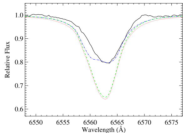
Figure 8. The mean observed H \alpha profile of \xi Per (solid, black) is well fitted by a wind model that has the low, X-ray-derived mass-loss rate, of 2.2 \times 10^{-7} M_{\odot} \text{ yr}^{-1} , and f_{\text{cl}} = 20 with a clumping onset, R_{\text{cl}} , just above the photosphere (dot-dashed, blue). Neither an unclumped model (dotted red) nor a model with f_{\text{cl}} = 20 but a clumping onset of R_{\text{cl}} = 1.3 R_* (dashed green) fits the data.
