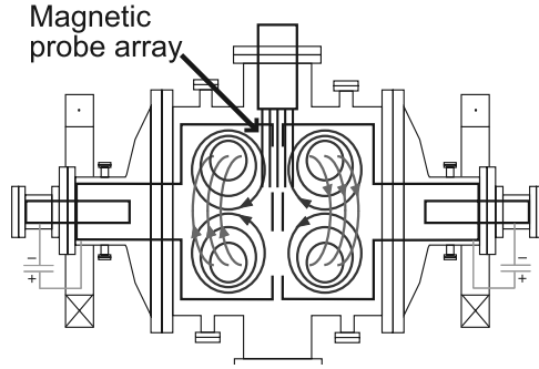
Figure 1. Diagram of the SSX device showing the location of the magnetic probe array.
