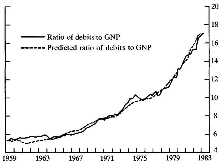
Figure A5.1. Actual and predicted transaction ratios.
