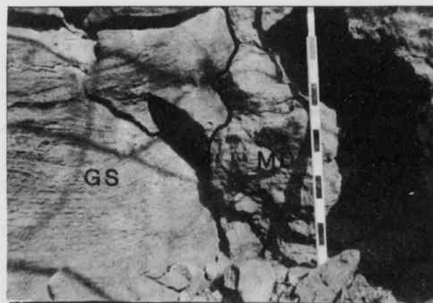
Figure 8. Abrupt facies boundary between simultaneously deposited mound rock (MD) and intermound grainstone (GS). This contact infers vertical mound accretion rates greater than that of the coevally sedimented intermound sediment. Also note the laminated cross beds of the grainstone demonstrating competent currents which are required to laminate sand sized skeletal particles.
