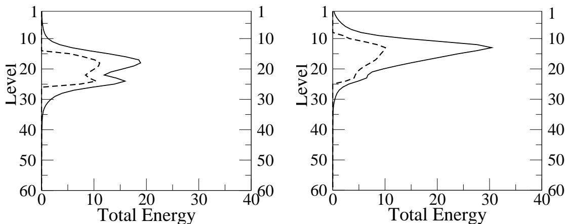
Fig A2: Vertical distribution of the mean total energy for the 10 leading S-SV's of JANUARY (default set), as a function of model level. Computed with an initial and final time projection operator that includes (a) levels 15–25, and (b) levels 10–25. The initial (final) time distribution is displayed by the dashed (solid) line. Final time energy is multiplied by a factor 0.1.
