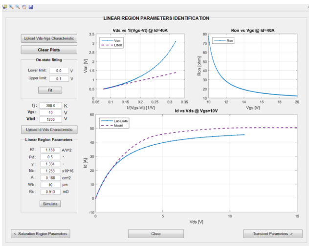
Fig. 5. MATLAB GUI panel for the identification of the linear region parameters
