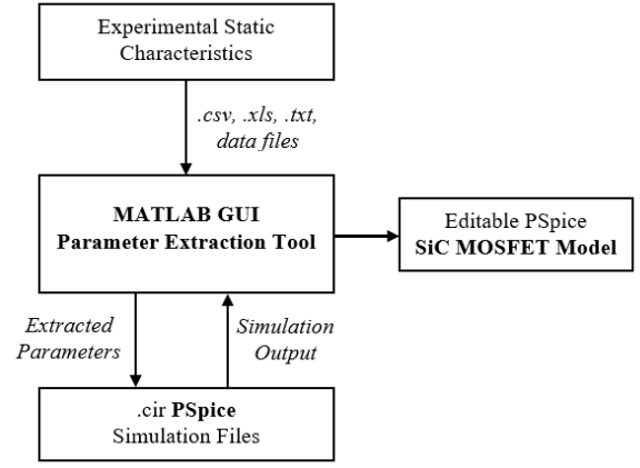
Fig. 2. Structure of the parameter extraction tool
