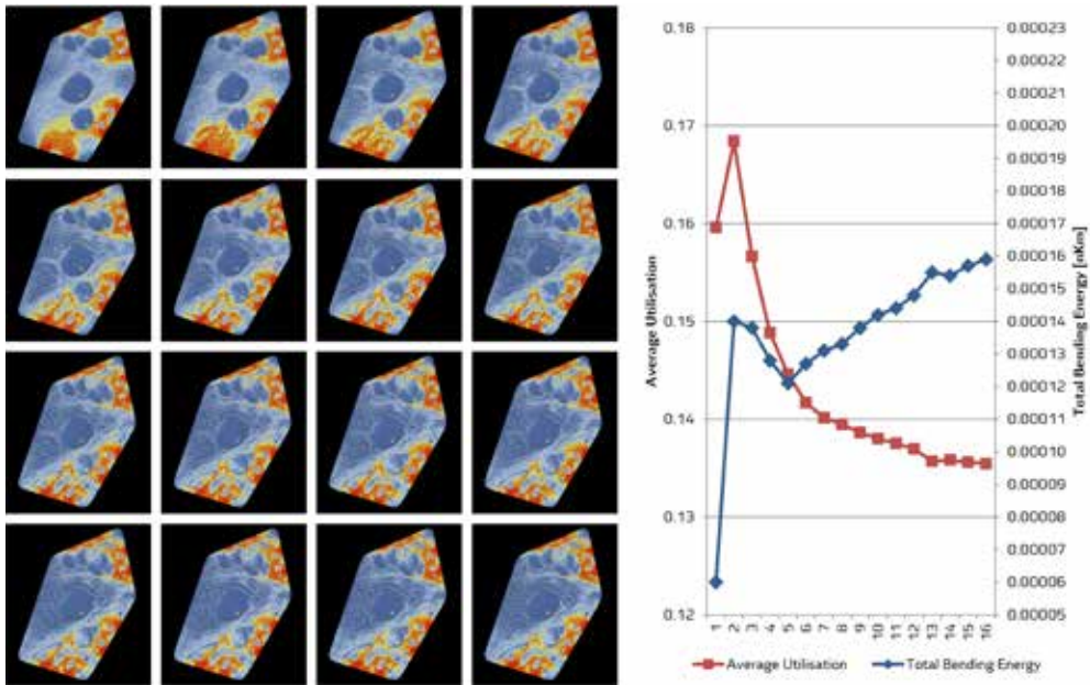
Figure 10: Reaction diffusion simulation run on global mesh to array upper skin patterning, then integrated with inter-skin connections and discretised for each unique panel.
