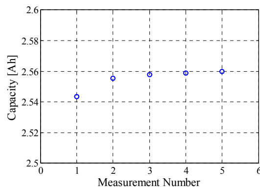
Figure 3. Discharging capacity of the LFP/C battery measured during the preconditioning test (1C-rate, T = 25 °C).
