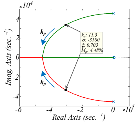
Fig. 3. Root locus for the inner current loop with P regulator, without voltage decoupling and neglecting system delays: x – open loop poles; ■ closed-loop poles for k_{pl} = 11.32 ; o – zeros
