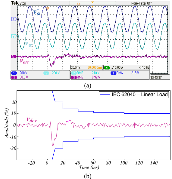
Fig. 13. Linear step load changing (0 – 100%): (a) reference (200 V/div), real (200 V/div), and capacitor voltage error (50 V/div) ( \alpha -axis), time scale (20 ms/div); (b) Dynamic characteristics according to IEC 62040 standard for linear loads
