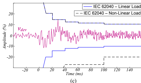
Fig. 10. Voltage loop with 5 th , 7 th HC and nonlinear load: (a) Step load changing (0 - 100%), reference (200 V/div), real (200 V/div) and capacitor voltage error (50 V/div) ( \alpha -axis), time scale (20 ms/div); (b) FFT of the capacitor voltage (250 Hz/div); (c) Dynamic characteristics according to IEC 62040 standard for linear loads, capacitor voltage deviation
