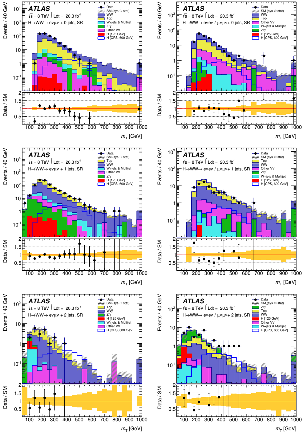
Figure 5. Transverse mass distributions in the 0-jet (top), 1-jet (middle) and \geq 2 jet (bottom) categories in the H \rightarrow WW \rightarrow l\nu l\nu signal regions. Different-flavour (left) and same-flavour (right) final states are shown. The histograms for the background processes, including the observed H[125 \text{ GeV}] , are shown stacked, and the distribution for a hypothetical CPS signal process with m_H = 600 \text{ GeV} and the cross section predicted by the SM for that mass is overlaid. The combined statistical and systematic uncertainties on the prediction are shown by the hatched band in the upper pane and the shaded band in the lower pane. In each figure, the last bin contains the overflow.
