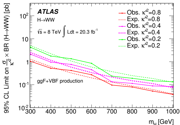
Figure 16. 95% CL upper limits in the intermediate-width scenario from the combination of the H \rightarrow WW \rightarrow \ell\nu\ell\nu and H \rightarrow WW \rightarrow \ell\nu q\bar{q} final states. Limits are set on \frac{\sigma_H}{\kappa^2} \times \text{BR}(H \rightarrow WW) for a heavy scalar resonance with a width in the range 0.2\Gamma_{H,\text{SM}} \leq \Gamma_H \leq 0.8\Gamma_{H,\text{SM}} . The ggF and VBF production modes have been combined.
