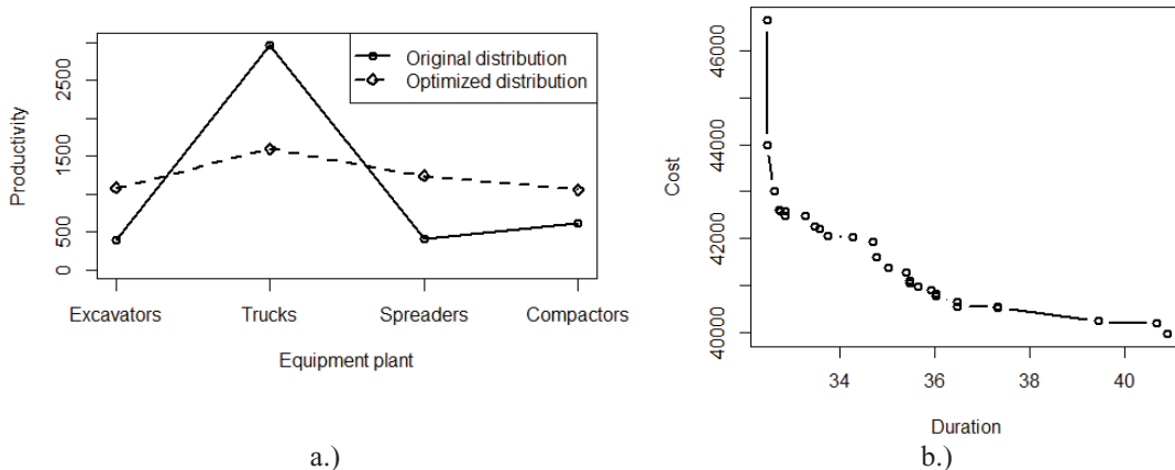
Figure 2: a.) Comparison between equipment productivity (in m 3 /h) in each task for the original equipment distribution and the optimized distribution solution; b.) Output of one run of the optimization system for the case-study (x-axis in hours, and y-axis in €)
