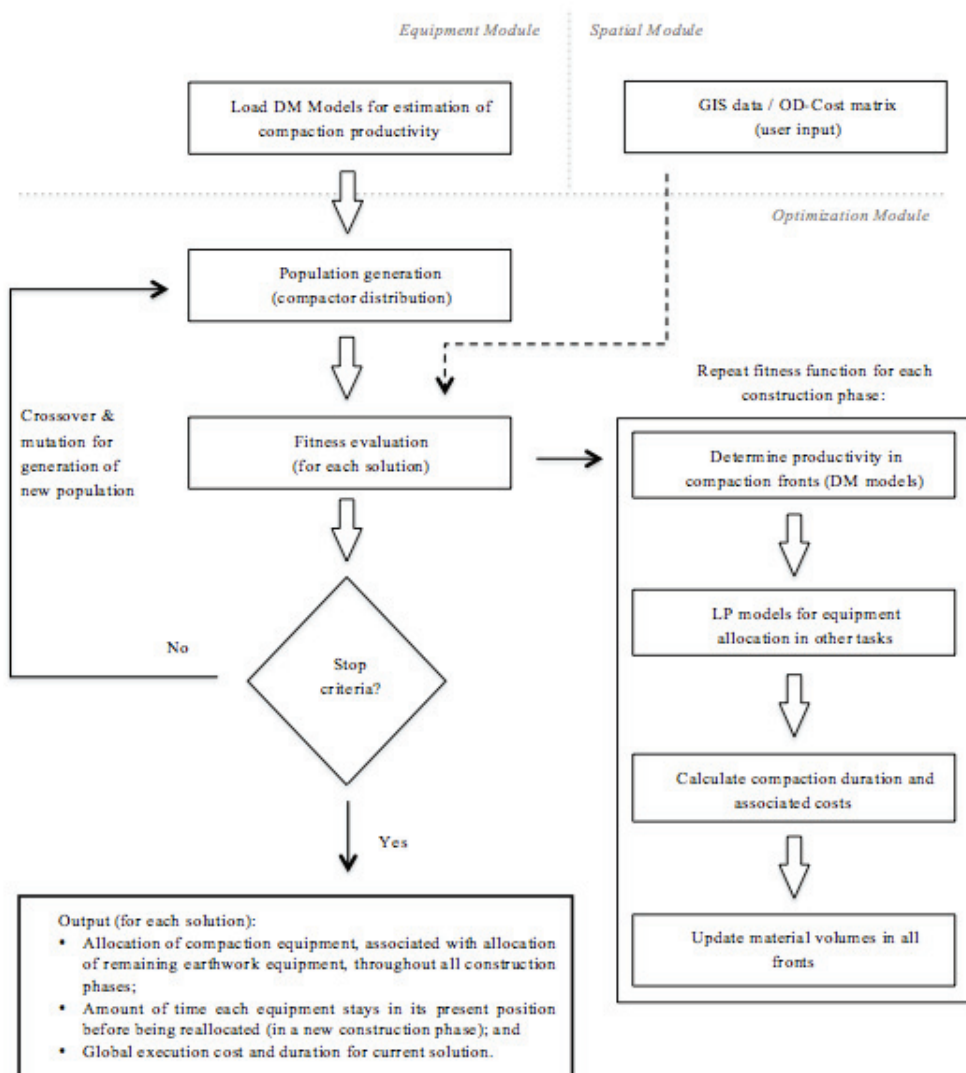
Figure 1: Integrated optimization system
