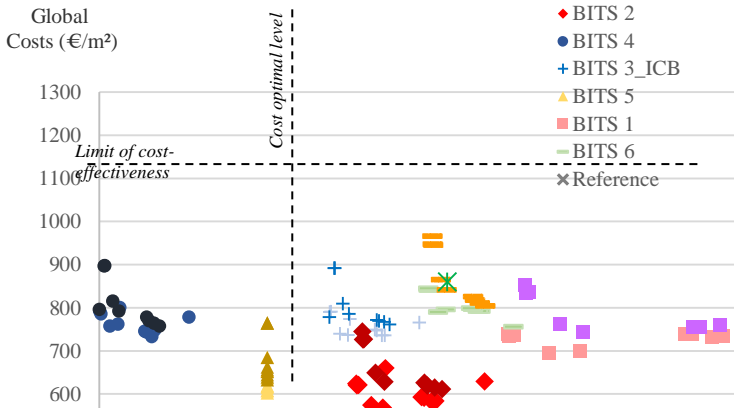
Figure 2. LCC analysis for all the renovation scenarios
