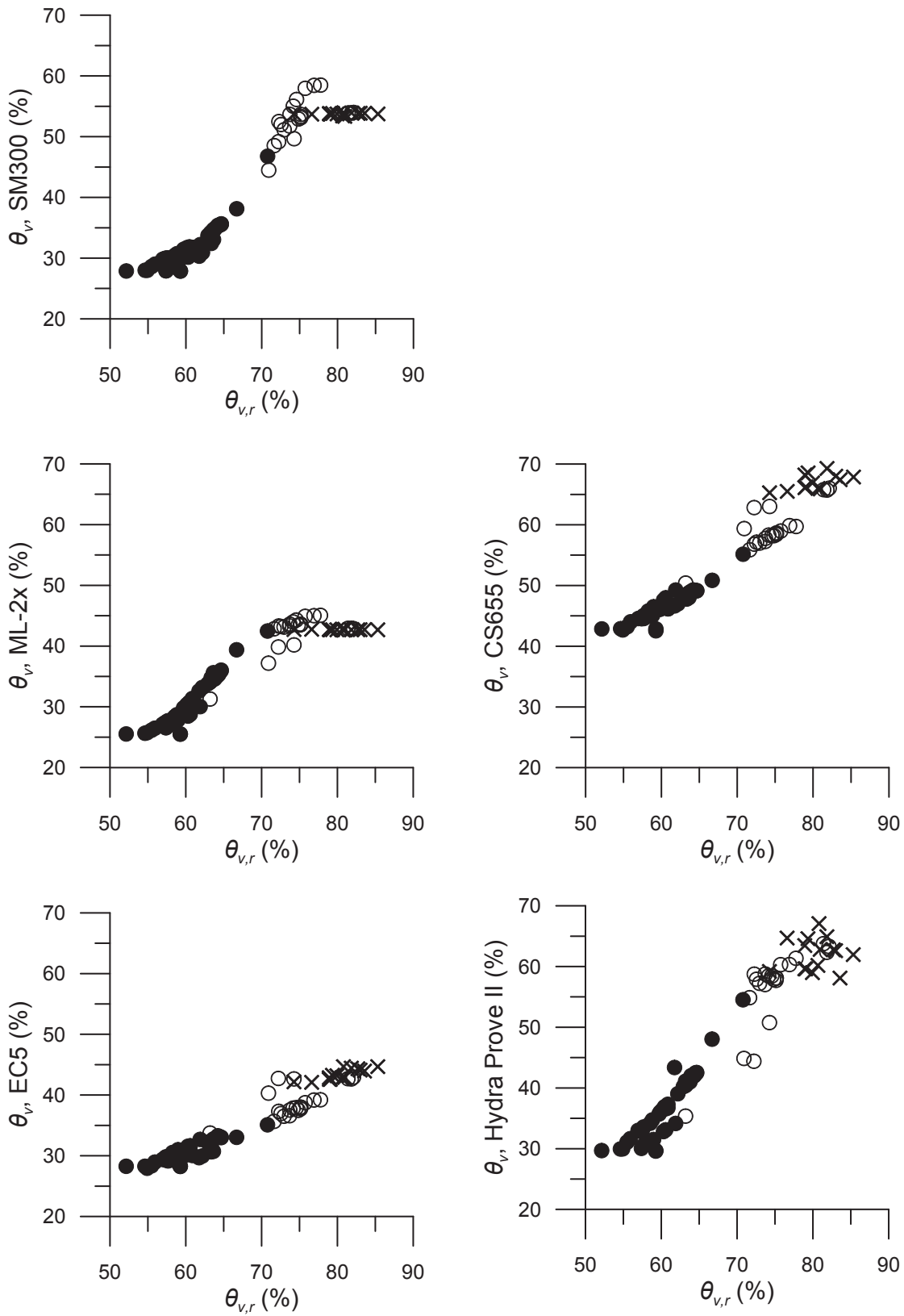
Fig. 2 Relation between the \theta_v values measured by the five sensors and the reference \theta_{v,r} values from the weight measurement. Closed circles indicate those for \text{bulk EC} \leq 1.5 \text{ dS/m} , open circles for 1.5 < \text{bulk EC} \leq 2.5 \text{ dS/m} , and crosses for 2.5 \text{ dS/m} < \text{bulk EC} .
