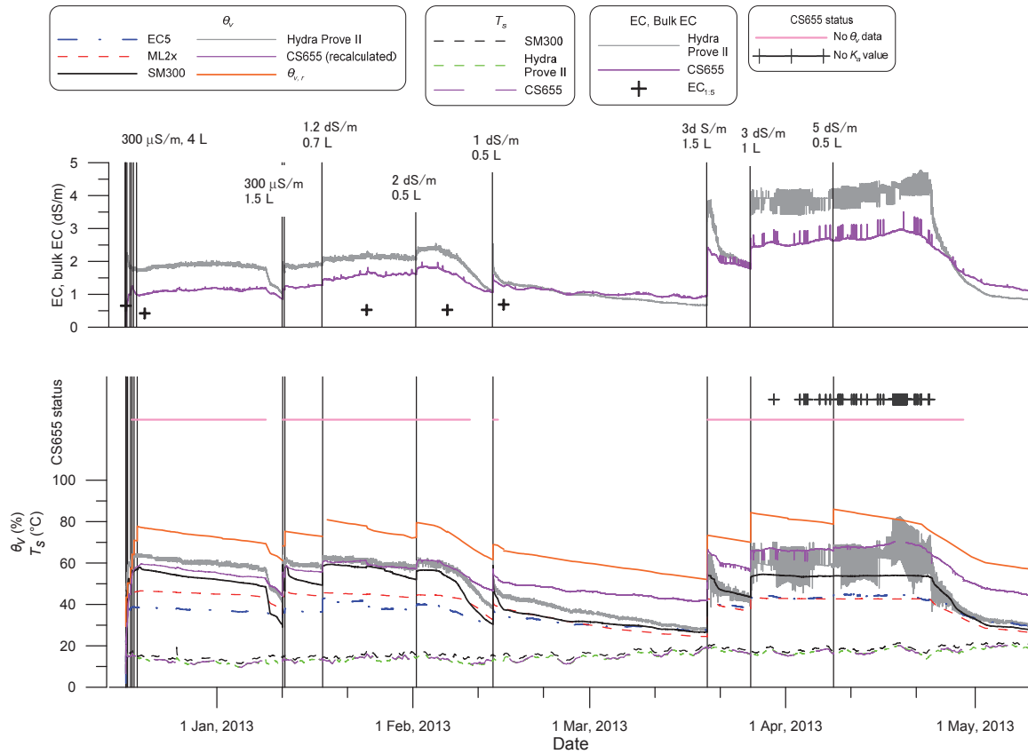
Fig. 1 Time changes of \theta_v measured by the five sensors, reference \theta_{v,r} from the weight measurement, the soil temperature T_s , the bulk EC measured by two sensors, the solution EC_{1,5} of the soil, and the status of the CS655 sensor observed in the experiment. Timings of the addition of salty water are shown by vertical lines, together with information on the EC value and amount.
